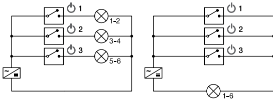
OR circuit
