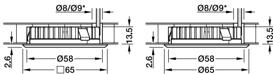
Recess mounting, square Lắp âm, vuông
